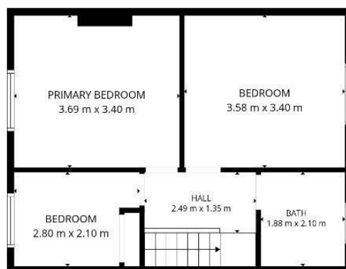
1st floor
